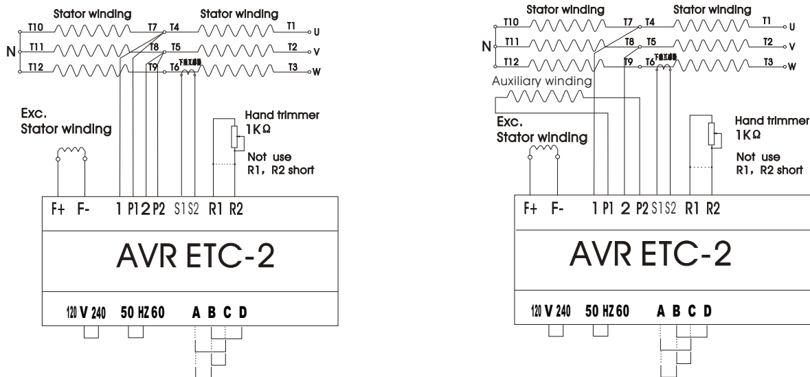
Typical wiring diagram of the three-phase four-wire, 380V voltage mode
